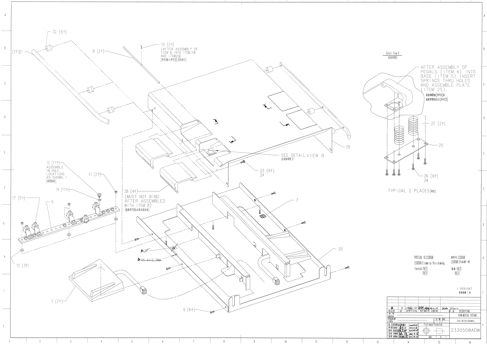
Figure 2-51 Footswitch Assembly (2330508 sheet 1, rev 2)
