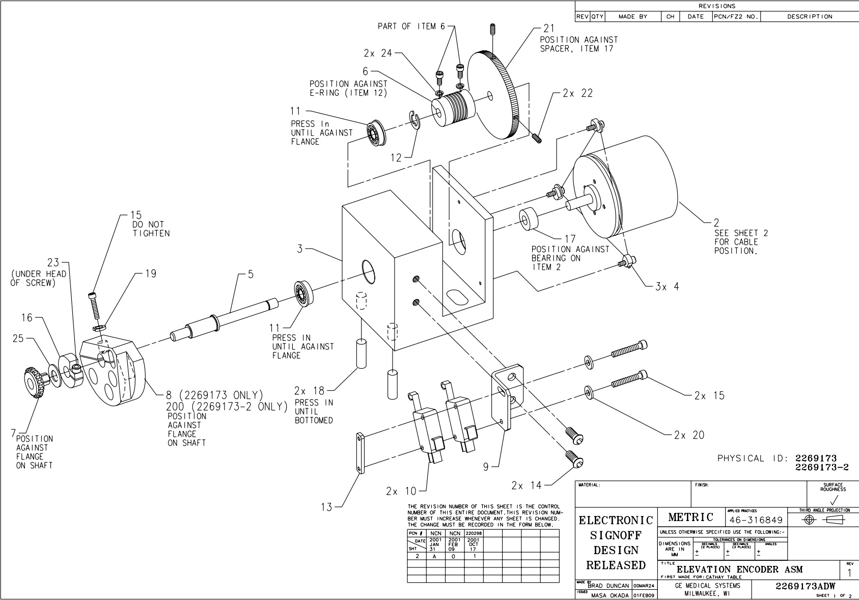
Figure 2-20 Elevation Encoder Assembly (2269173, sheet 1, rev 1)
