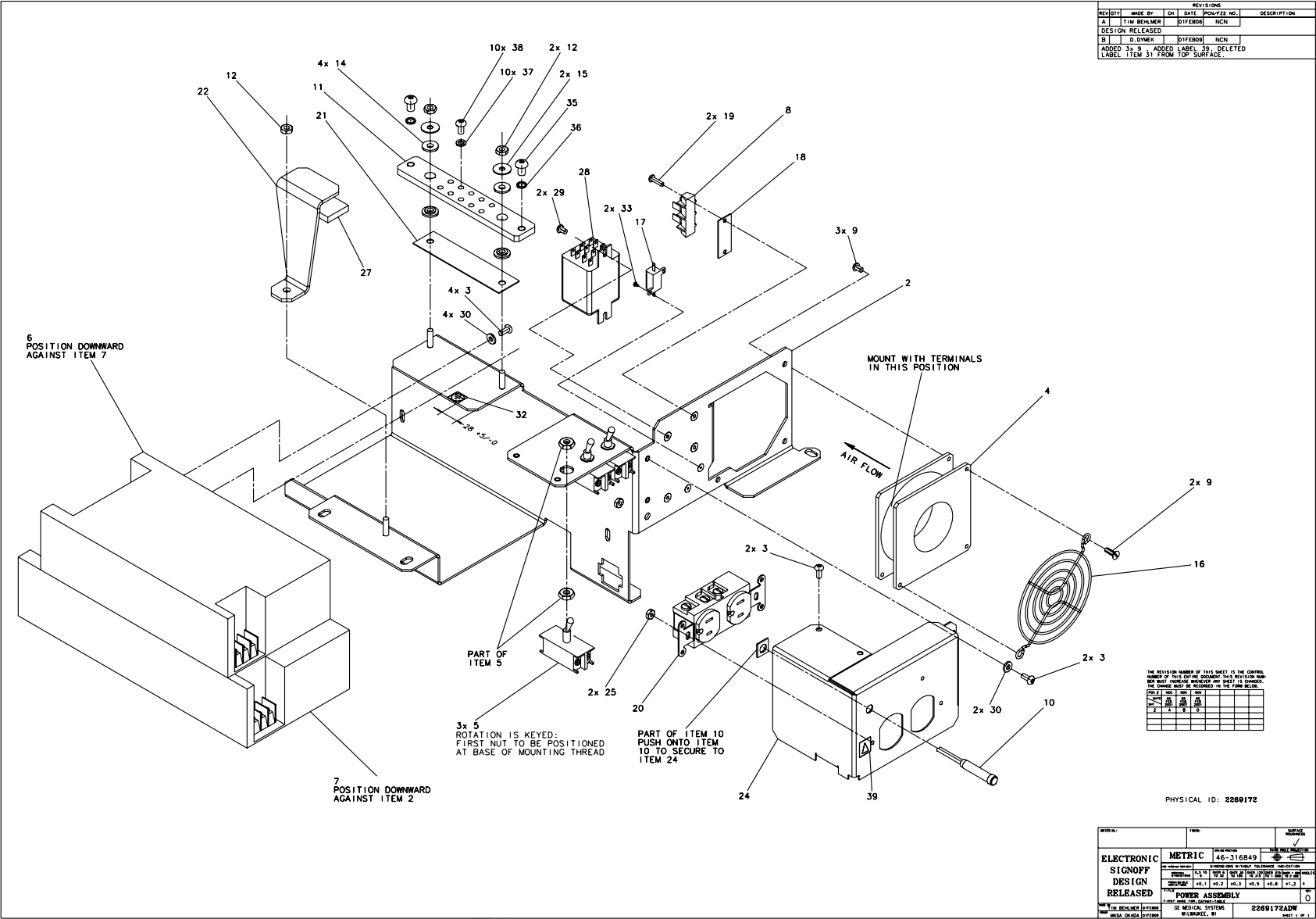
Figure 2-18 Power Supply Assembly (2269172, sheet 1, rev 0)
