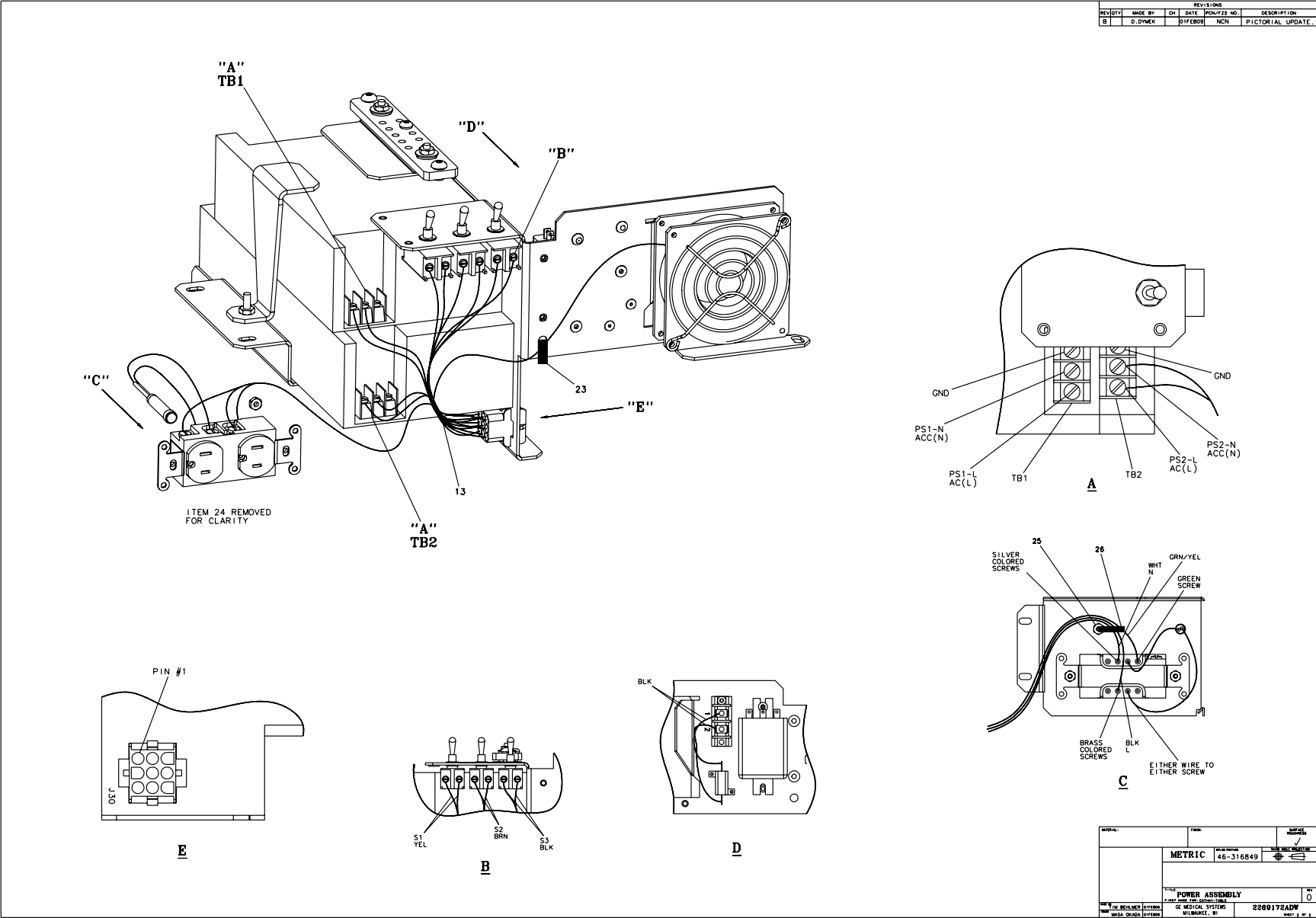
Figure 2-19 Power Supply Assembly (2269172, sheet 2, rev 0)
