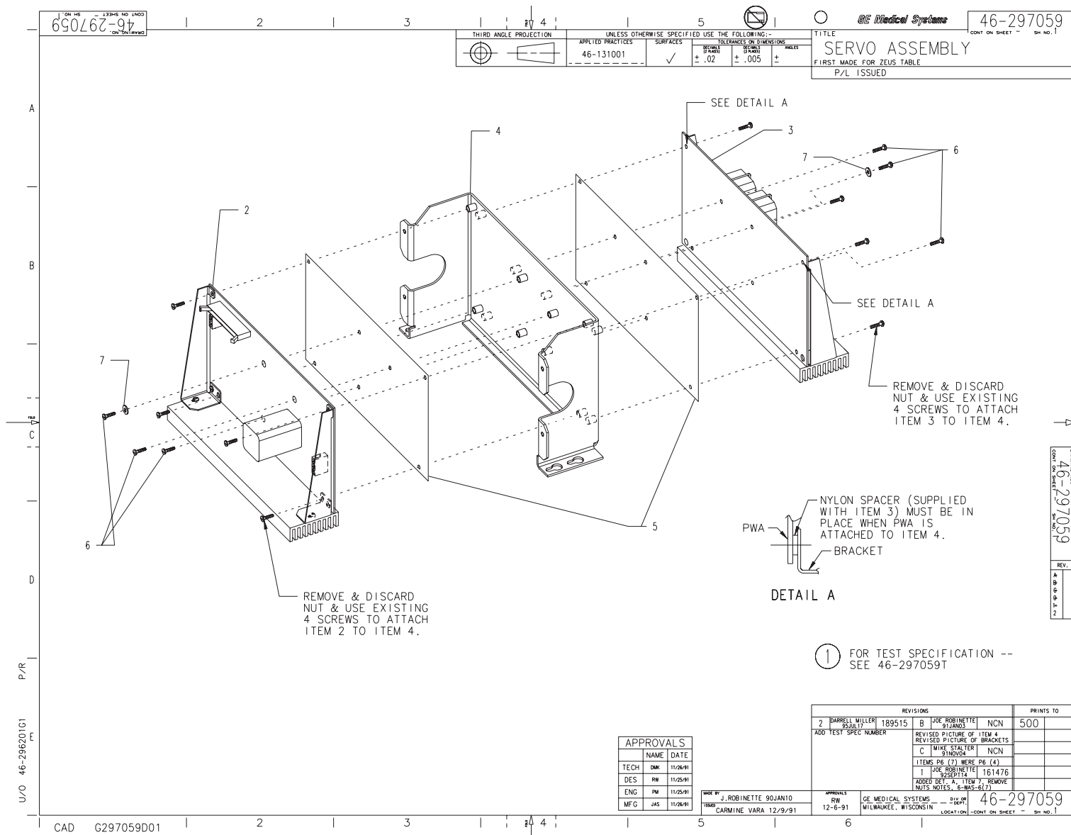
Figure 2-17 Servo Assembly (46-297059, sheet 1, rev 2)
