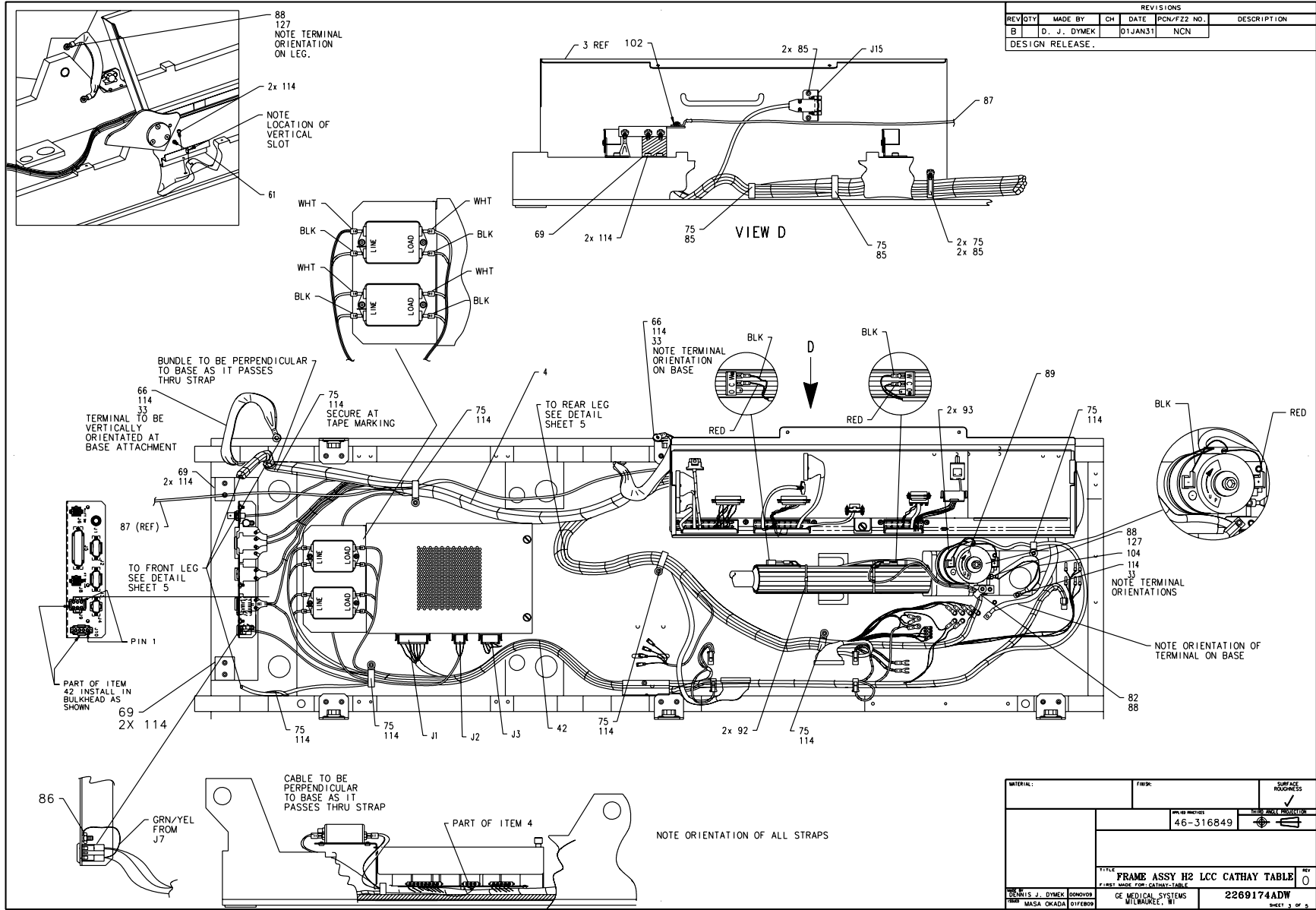
Figure 2-24 Frame Assembly (2269174, sheet 3, rev 0)
