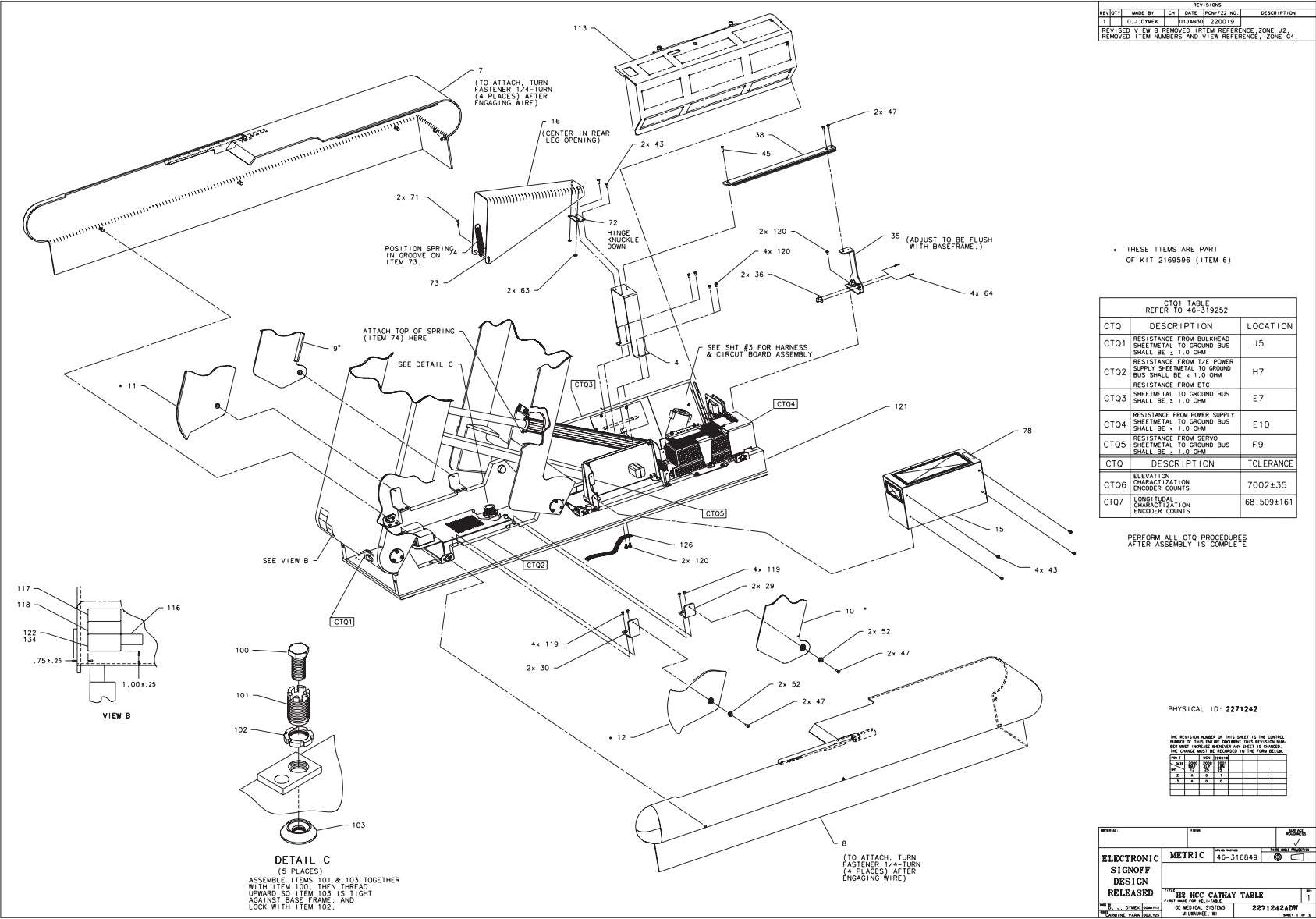
Figure 2-27 Table Assembly (2271242, sheet 1, rev 1)
