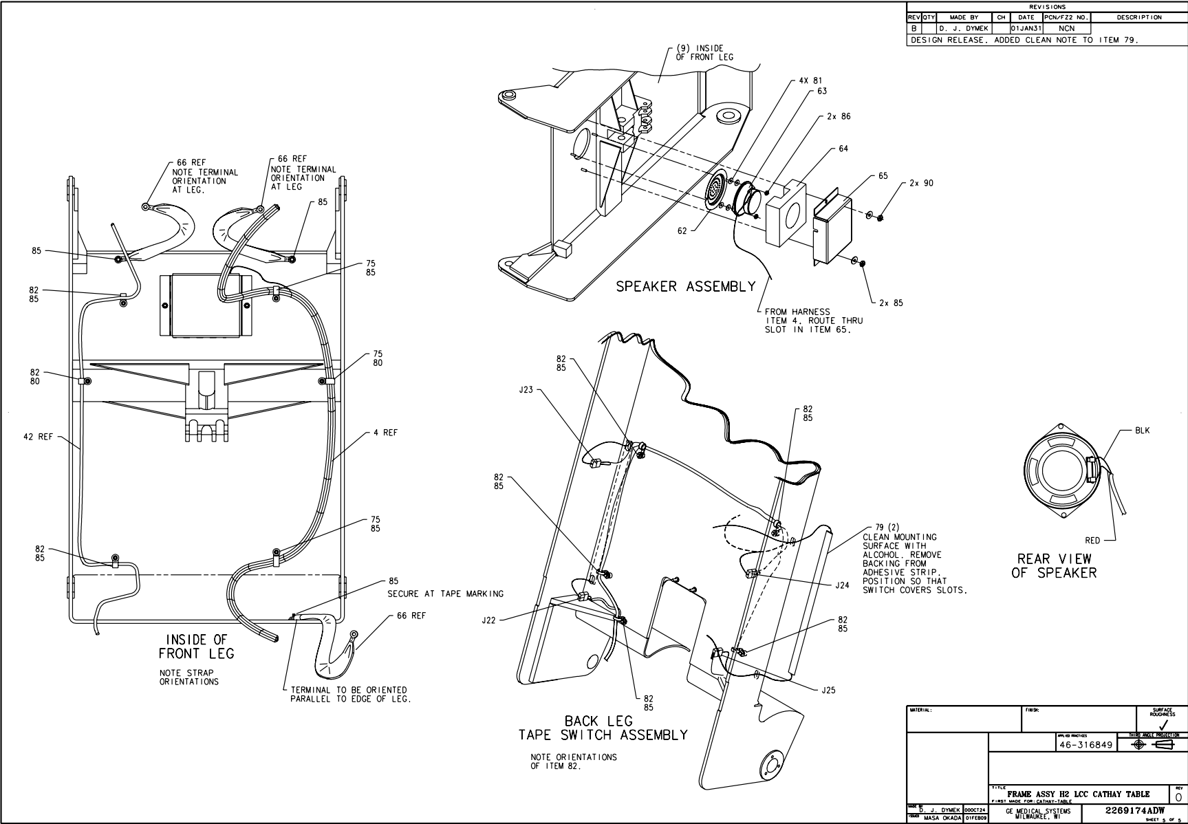
Figure 2-26 Frame Assembly (2269174, sheet 5, rev 0)
