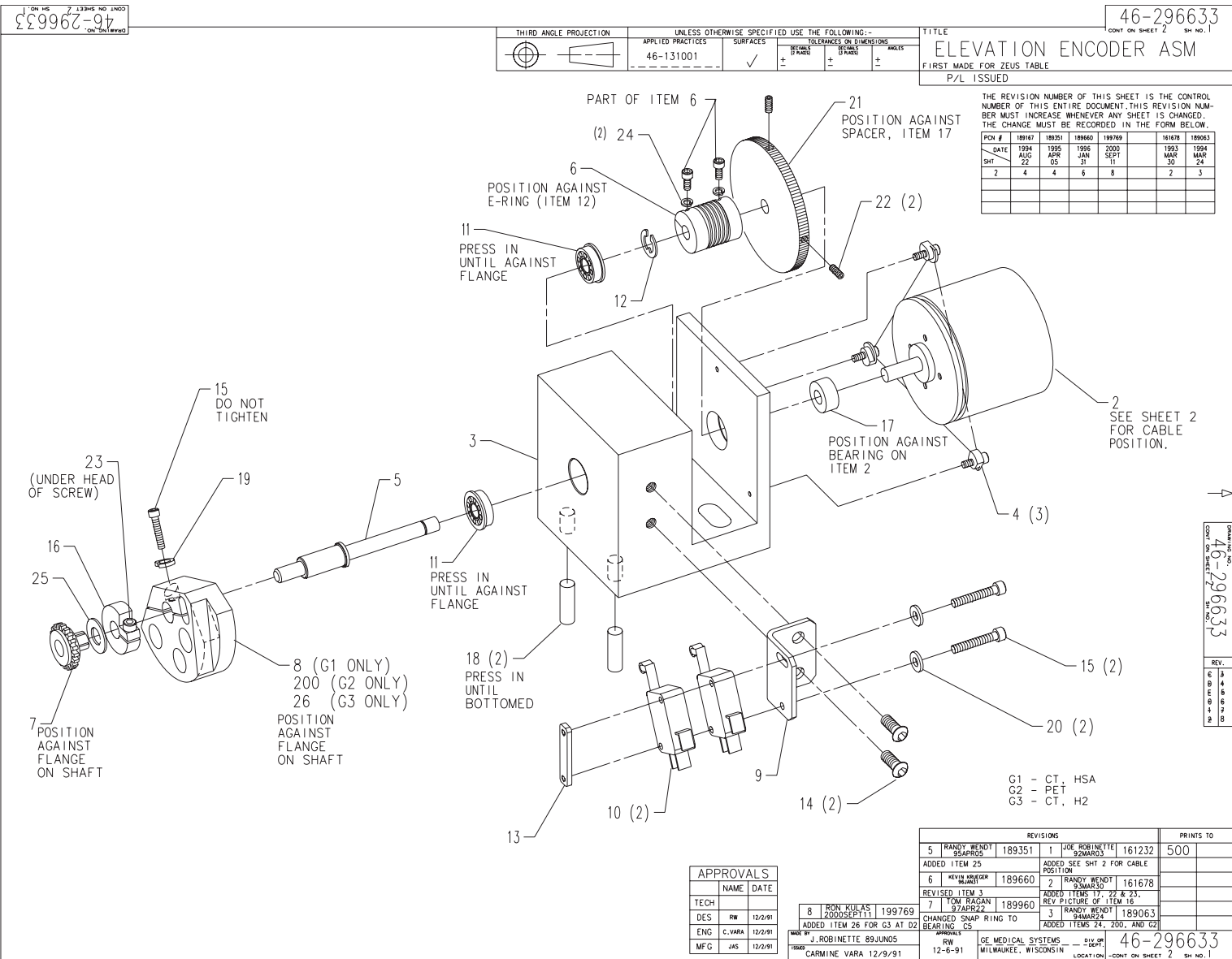
Figure 2-44 Elevation Encoder Assembly (46-296633G3, sheet 1, rev 8)
