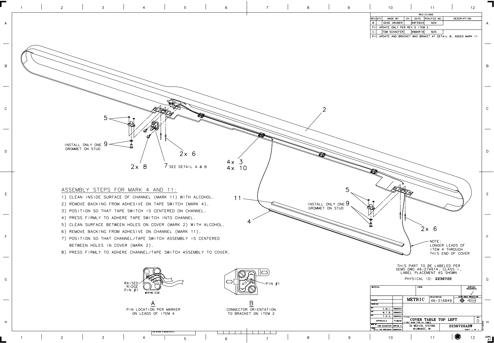
Figure 2-30 Cover Assembly Table Top - Left (2236720, sheet 1, rev 0)
