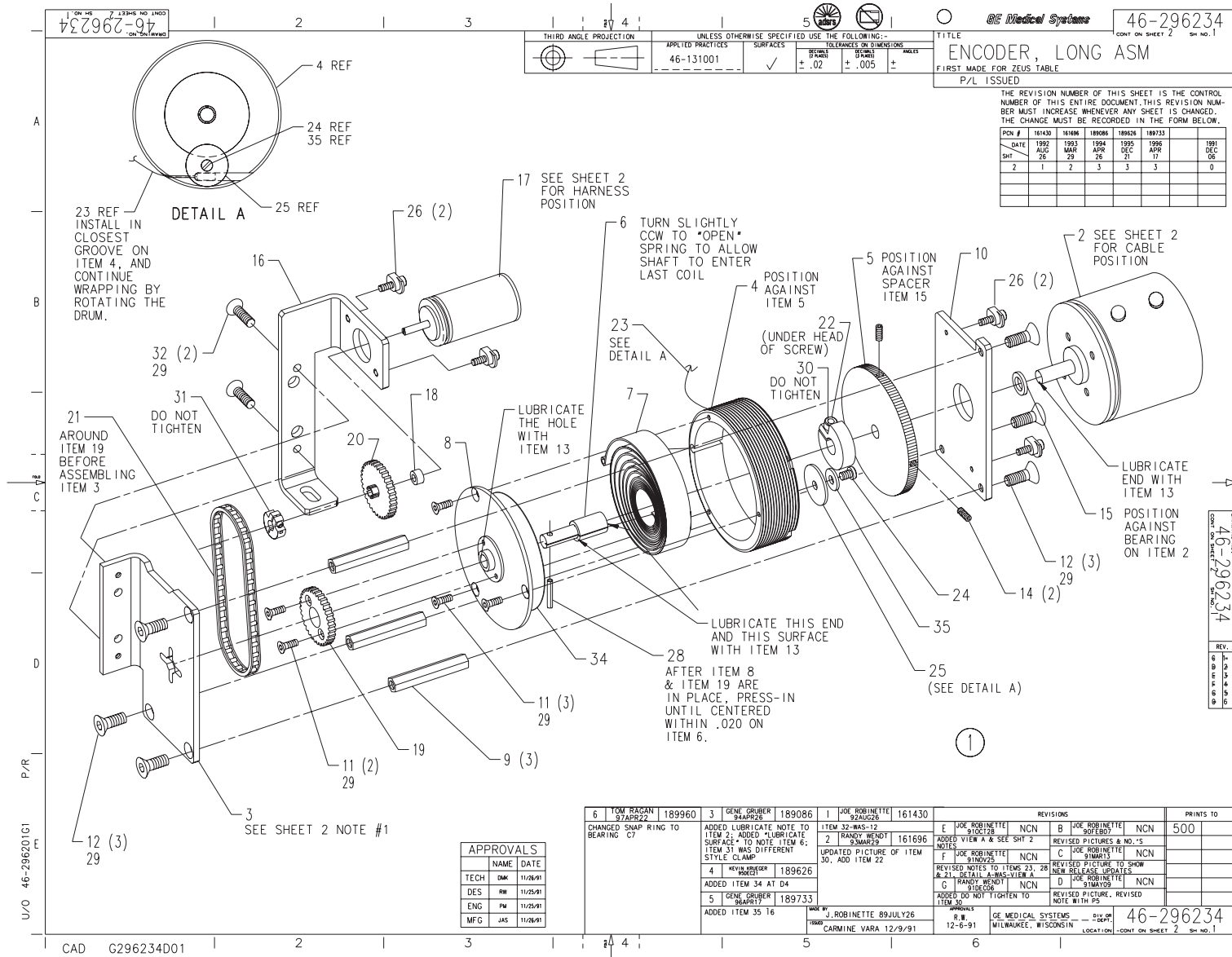
Figure 2-40 Table Encoder Assembly (46-296234, sheet 1, rev 6)
