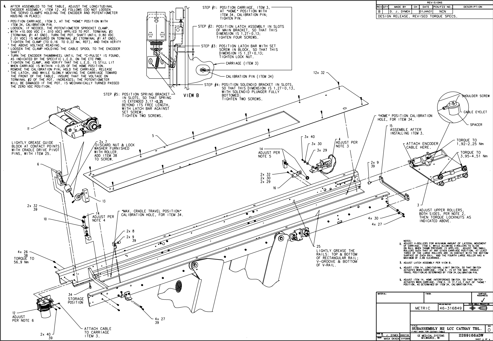
Figure 2-8 Table Subassembly (2269166, sheet 2, rev 0)
