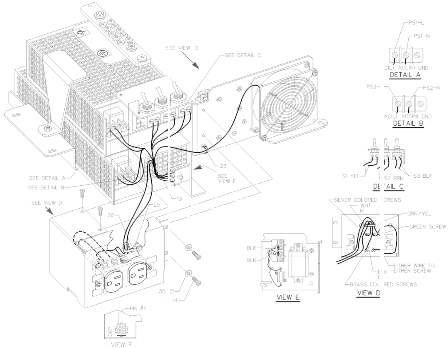
Figure 2-43 Power Assembly (46-296791, sheet 2, rev 8)
