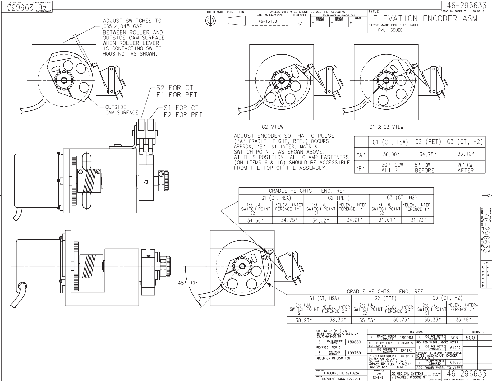
Figure 2-45 Elevation Encoder Assembly (46-296633G3, sheet 2, rev 8)
