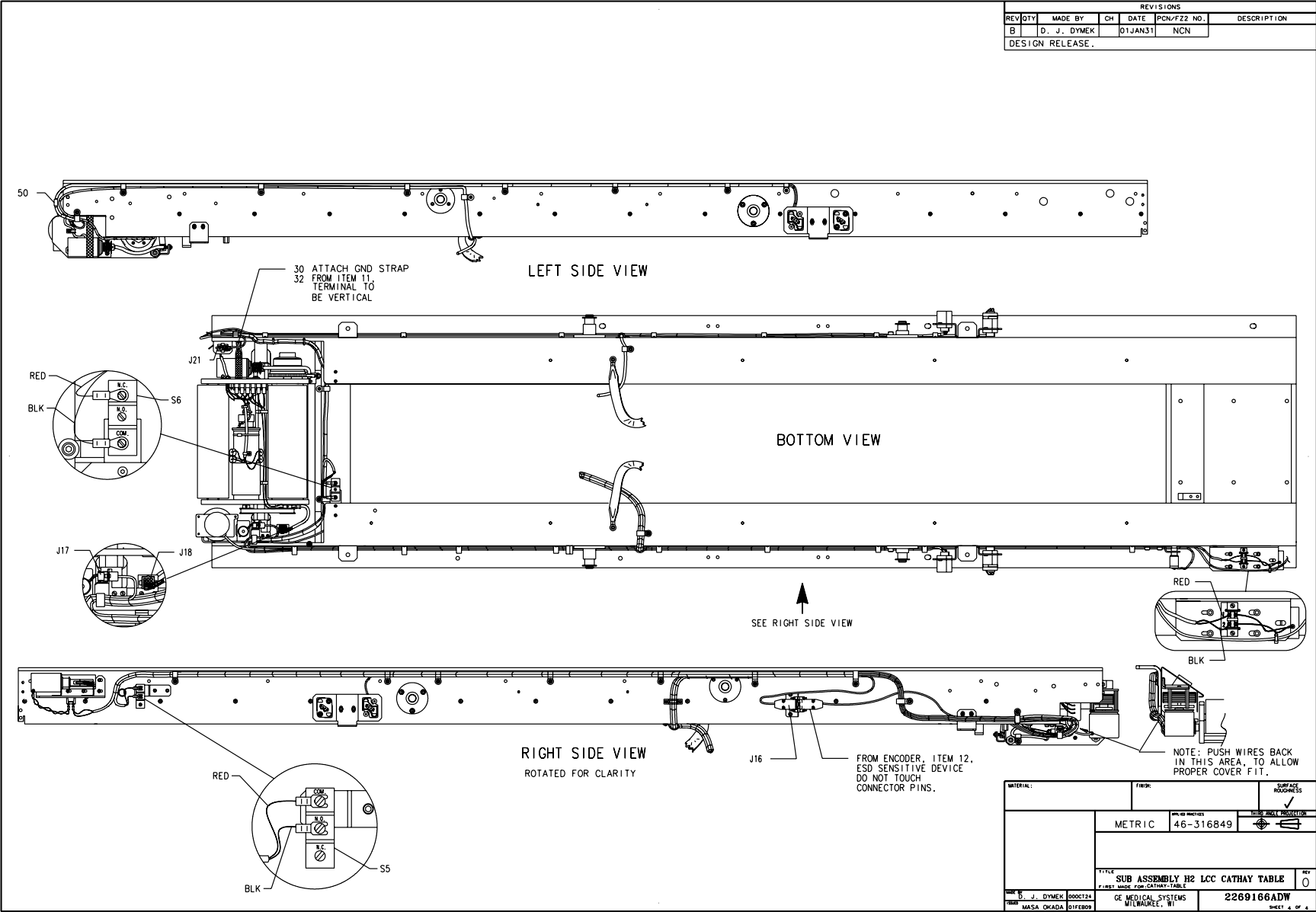
Figure 2-10 Table Subassembly (2269166, sheet 4, rev 0)
