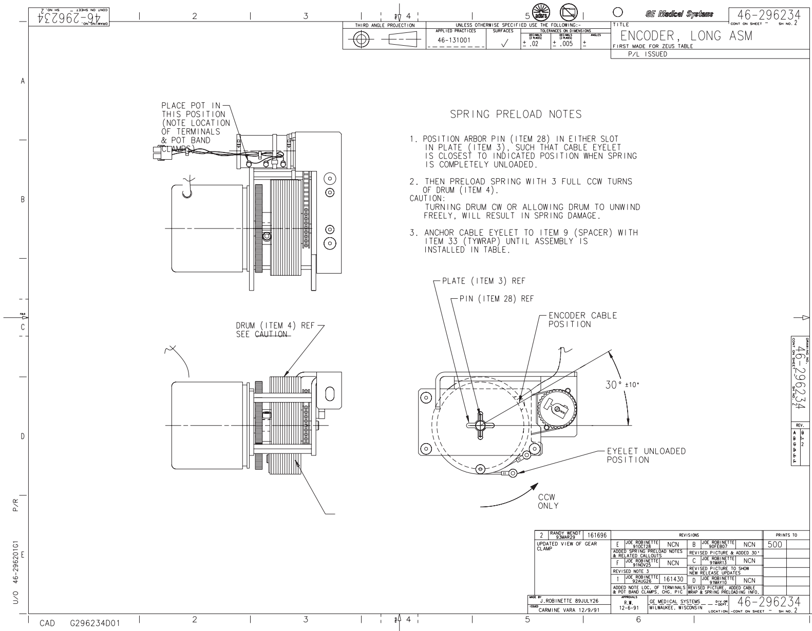
Figure 2-41 Table Encoder Assembly (46-296234, sheet 2, rev 2)
