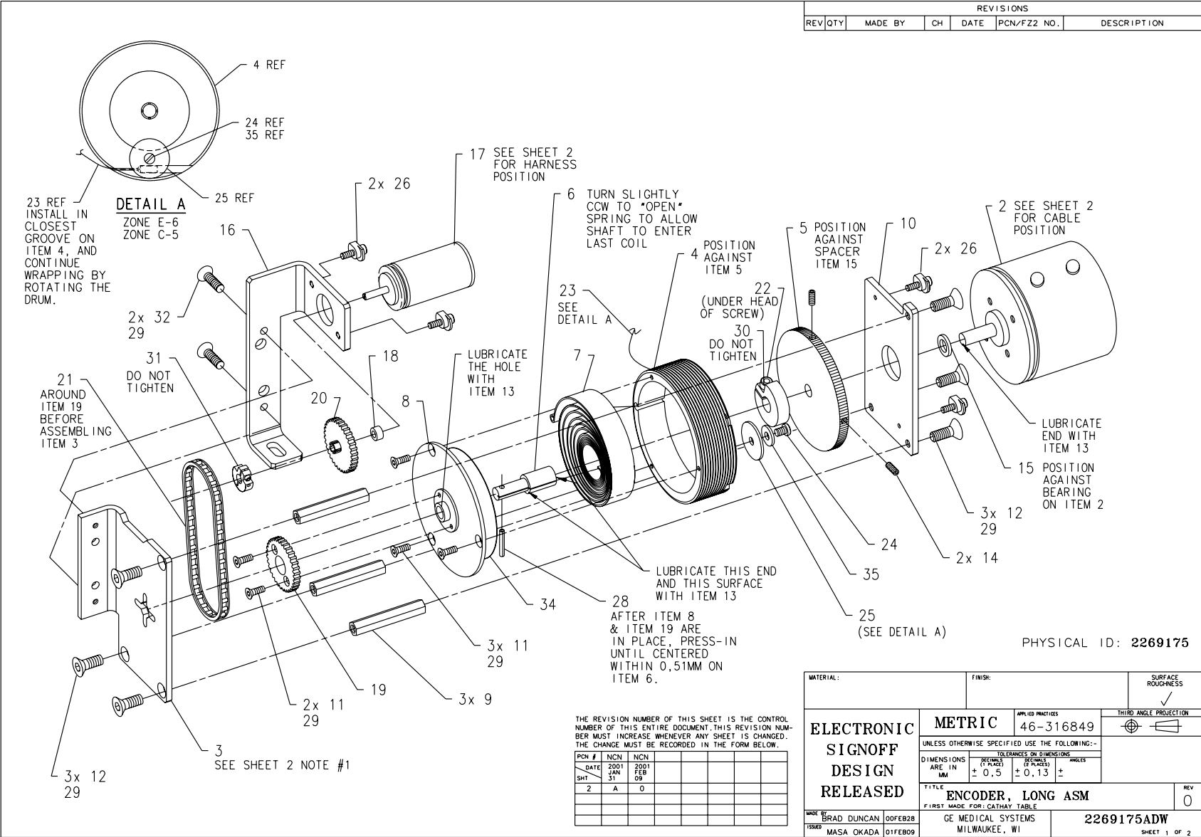
Figure 2-15 Longitudinal Encoder Asm (2269175, sheet 1, rev 0)
