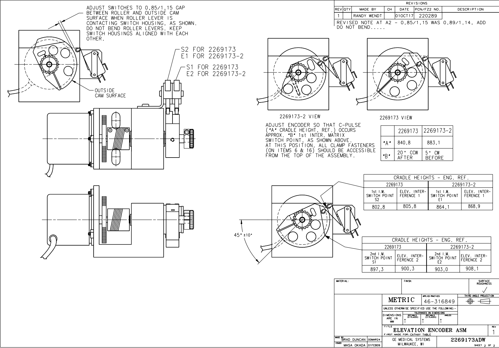
Figure 2-21 Elevation Encoder Assembly (2269173, sheet 2, rev 1)
