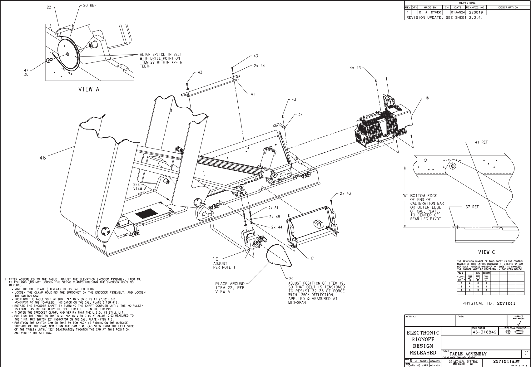
Figure 2-32 Subassembly For H2 HCC Cathay Table (2271241, sheet 1, rev 1)
