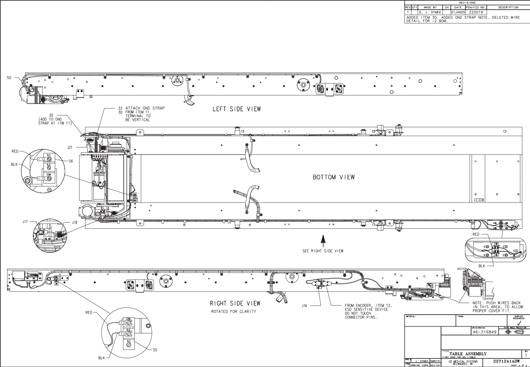
Figure 2-35 Subassembly For H2 HCC Cathay Table (2271241, sheet 4, rev 1)
