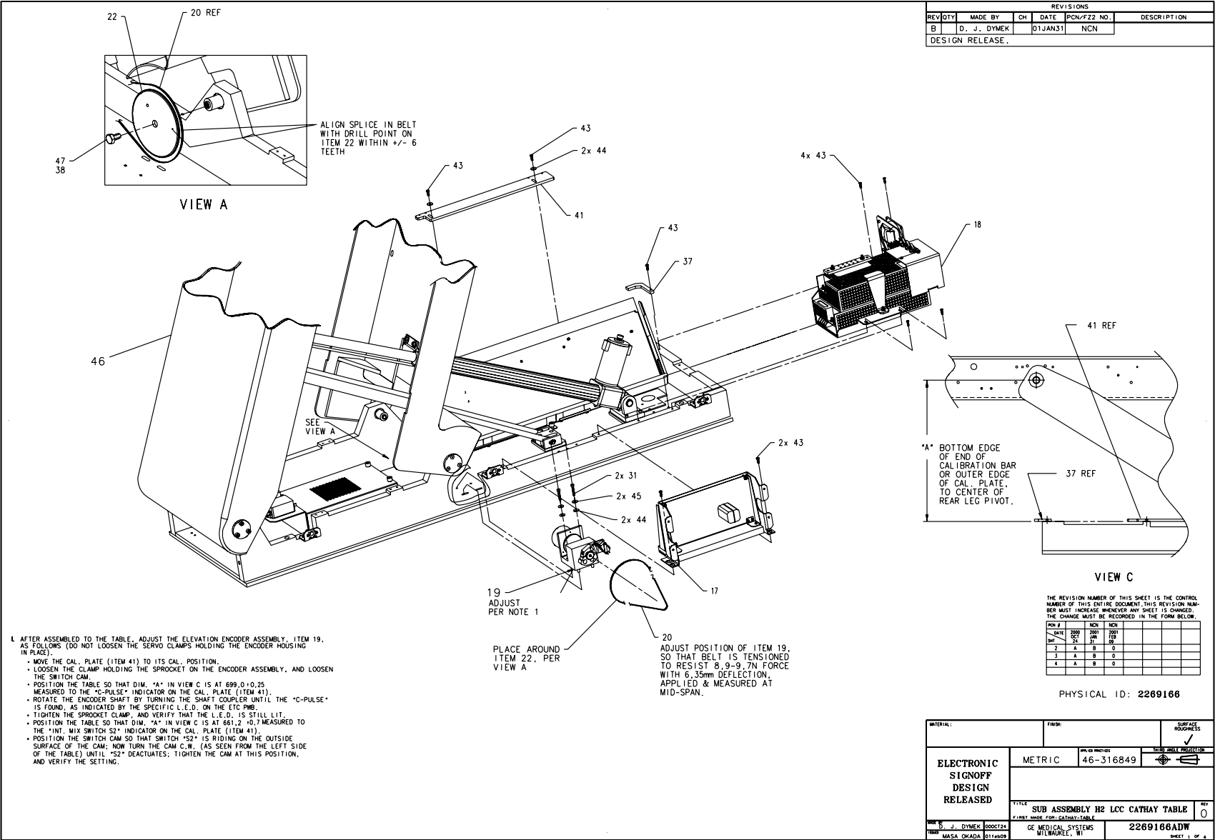
Figure 2-7 Table Subassembly (2269166, sheet 1, rev 0)
