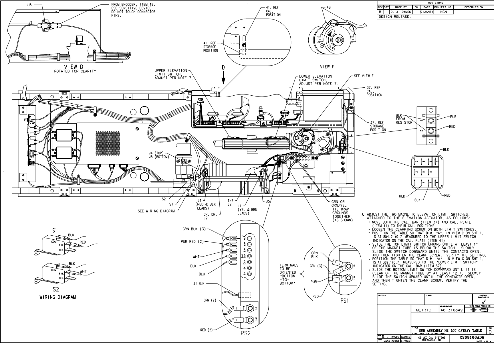
Figure 2-9 Table Subassembly (2269166, sheet 3, rev 0)
