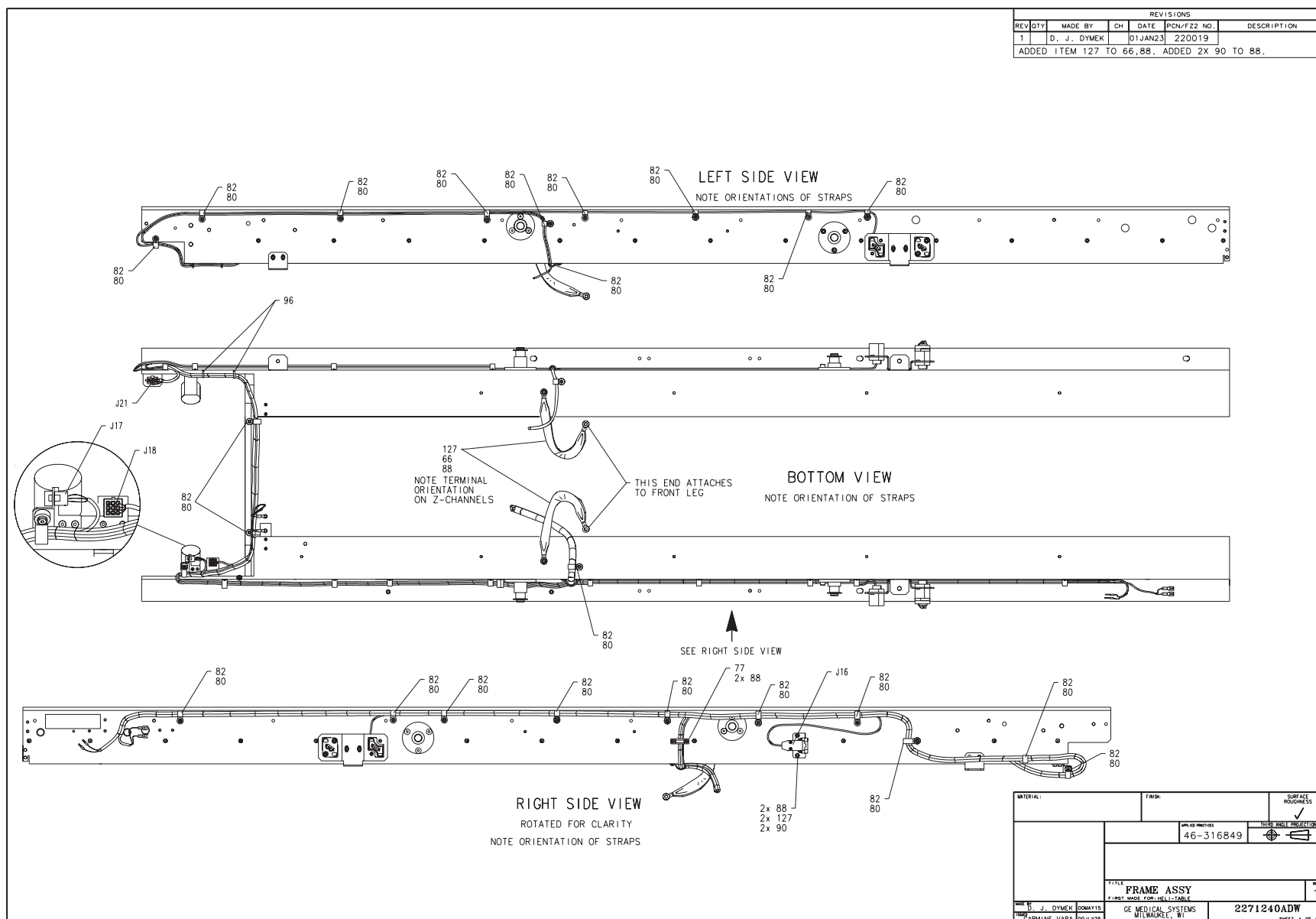
Figure 2-49 Frame Assembly, Table (2271240, sheet 4, rev 1)
