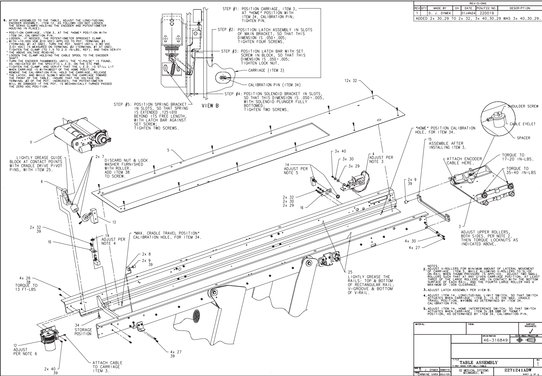
Figure 2-33 Subassembly For H2 HCC Cathay Table (2271241, sheet 2, rev 1)
