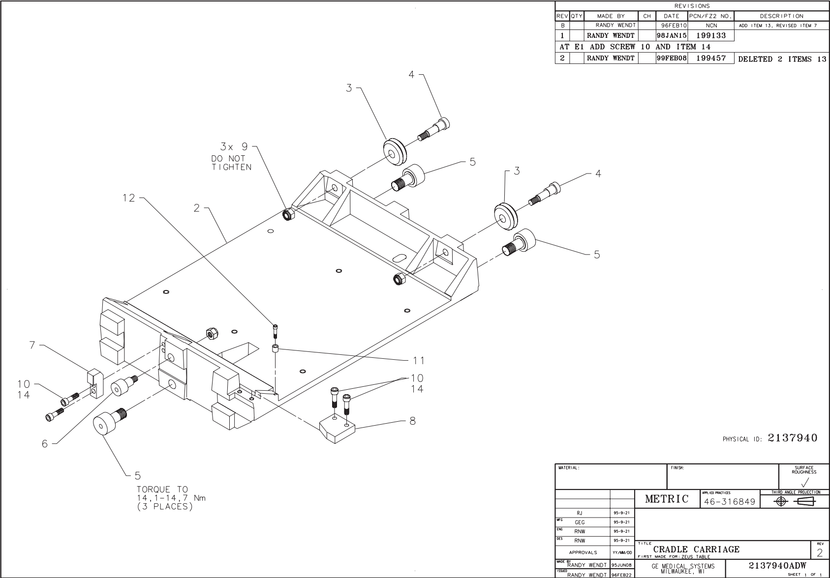
Figure 2-36 3 Point Carriage Assembly (2137940, sheet 1, rev 2)
