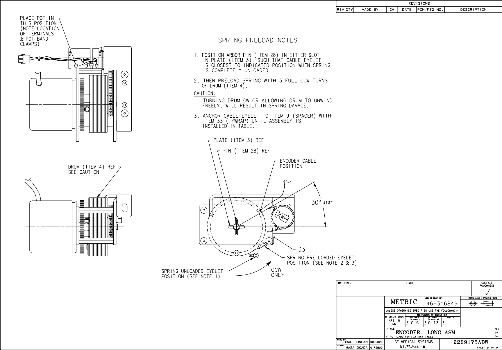
Figure 2-16 Longitudinal Encoder Asm (2269175, sheet 2, rev 0)
